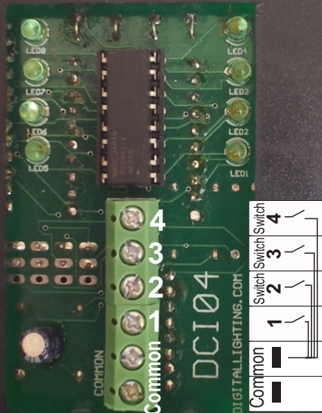
DCI04 Dry contact Switches Inputs
