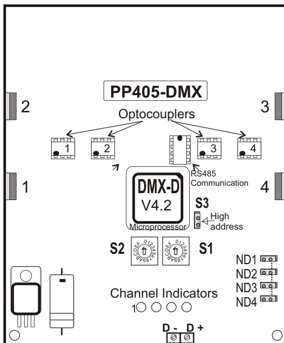
Figure 6 - PP405-DMX Address & Mode Selection.
