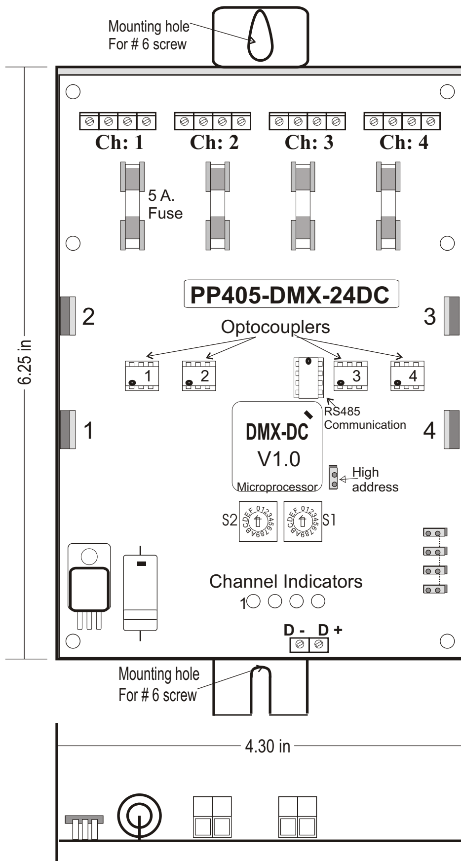
Figure 2 - PP405-DMX Dimensional Diagram
