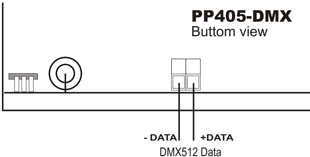
Figure 3 PP Dimmer Network Ports Connections.
