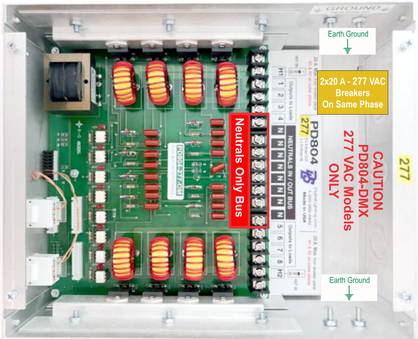
Figure 4. PD804-DMX Typical 277 VAC Wiring.
