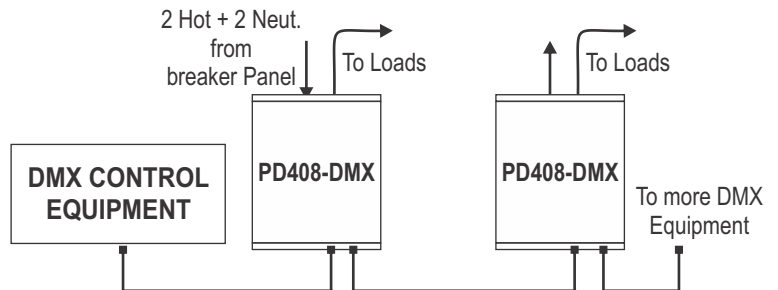
Figure 2 - Typical Installation
