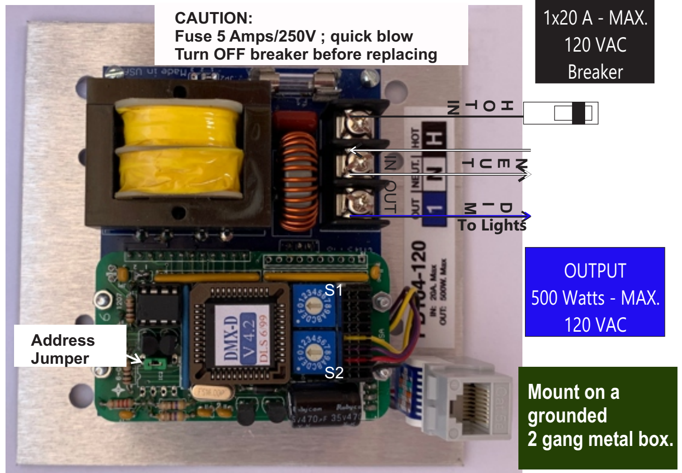
Figure 5 - PD104-DMX-120 Typical 120 VAC Wiring.
