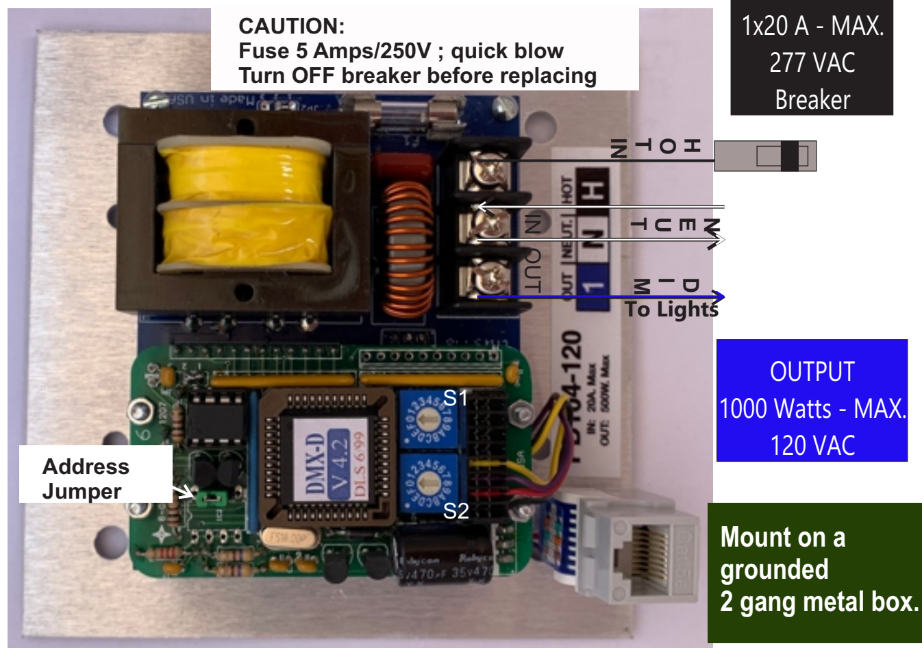
Figure 5 - PD104-DMX-277 Typical 277 VAC Wiring.
