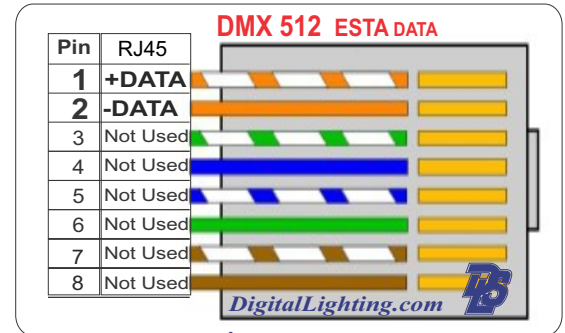
Figure 5 - PD104-DMX-277 Typical 277 VAC Wiring.
