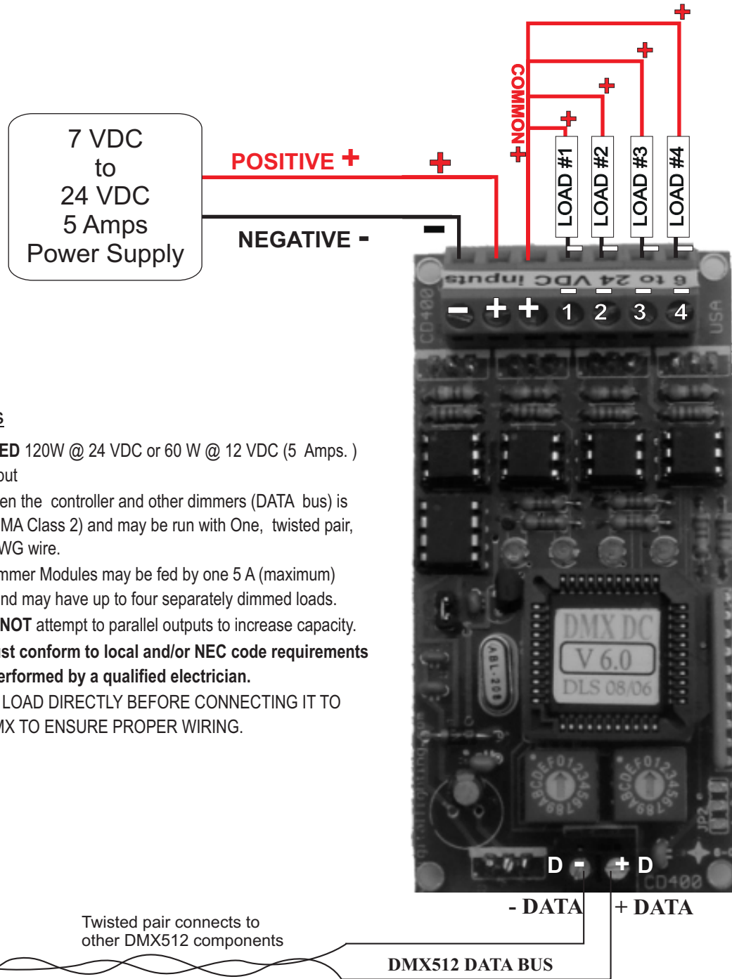
Figure 6 - Cd45 GENERAL WIRING INSTRUCTIONS:
