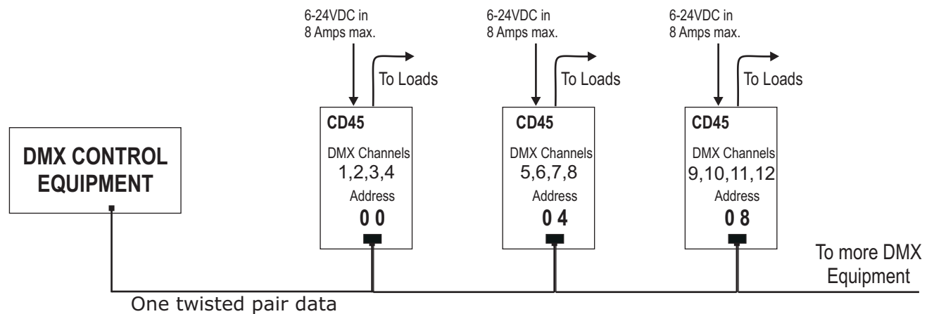
Figure 5 - Typical Installation
