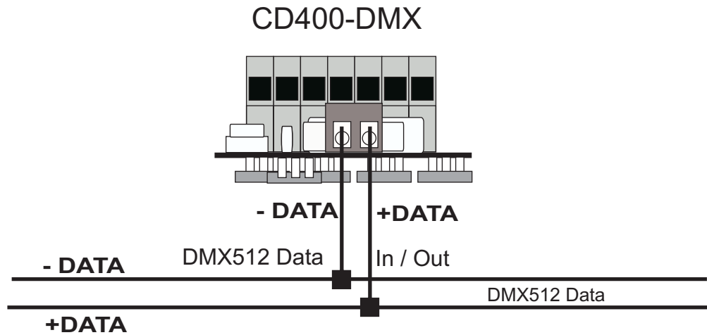
Figure 4 CD Dimmer DMX512 signal Connections.
