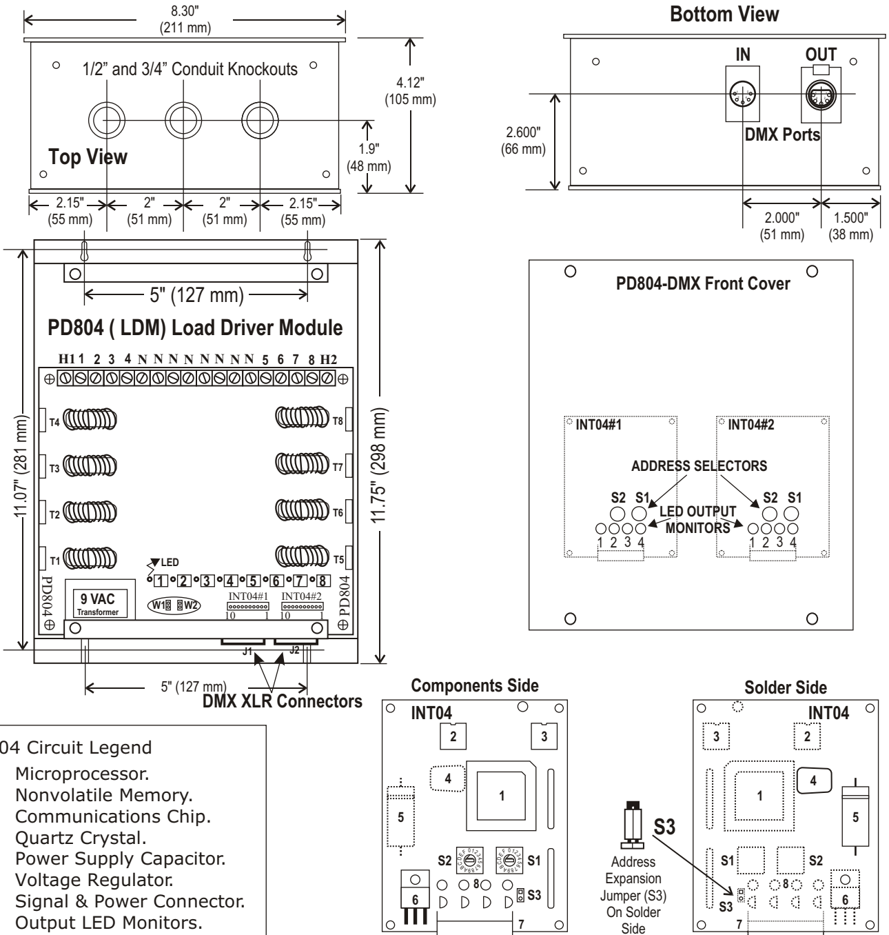
Figure 3. PD804-DMX Enclosure And Circuit Details
