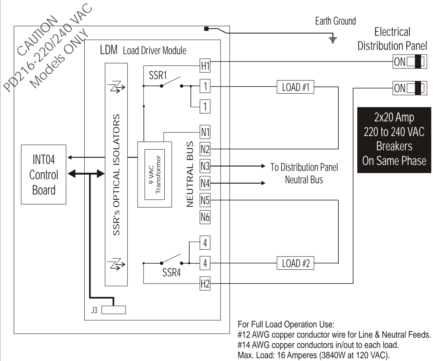
Figure 6 - PD216 Typical 220/240 VAC Wiring.
