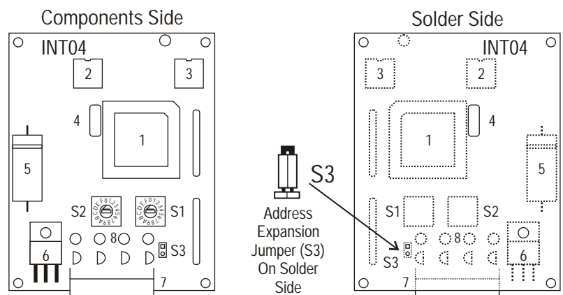
Figure 2 - PD216-DMX INT04 Detail
