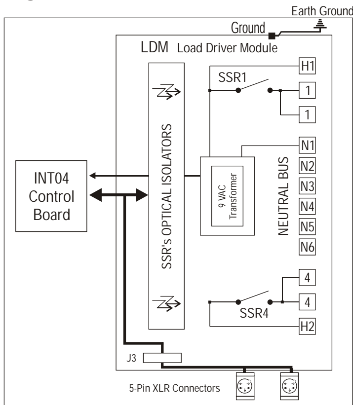
Figure 1 - PD216-DMX LDM Detail
