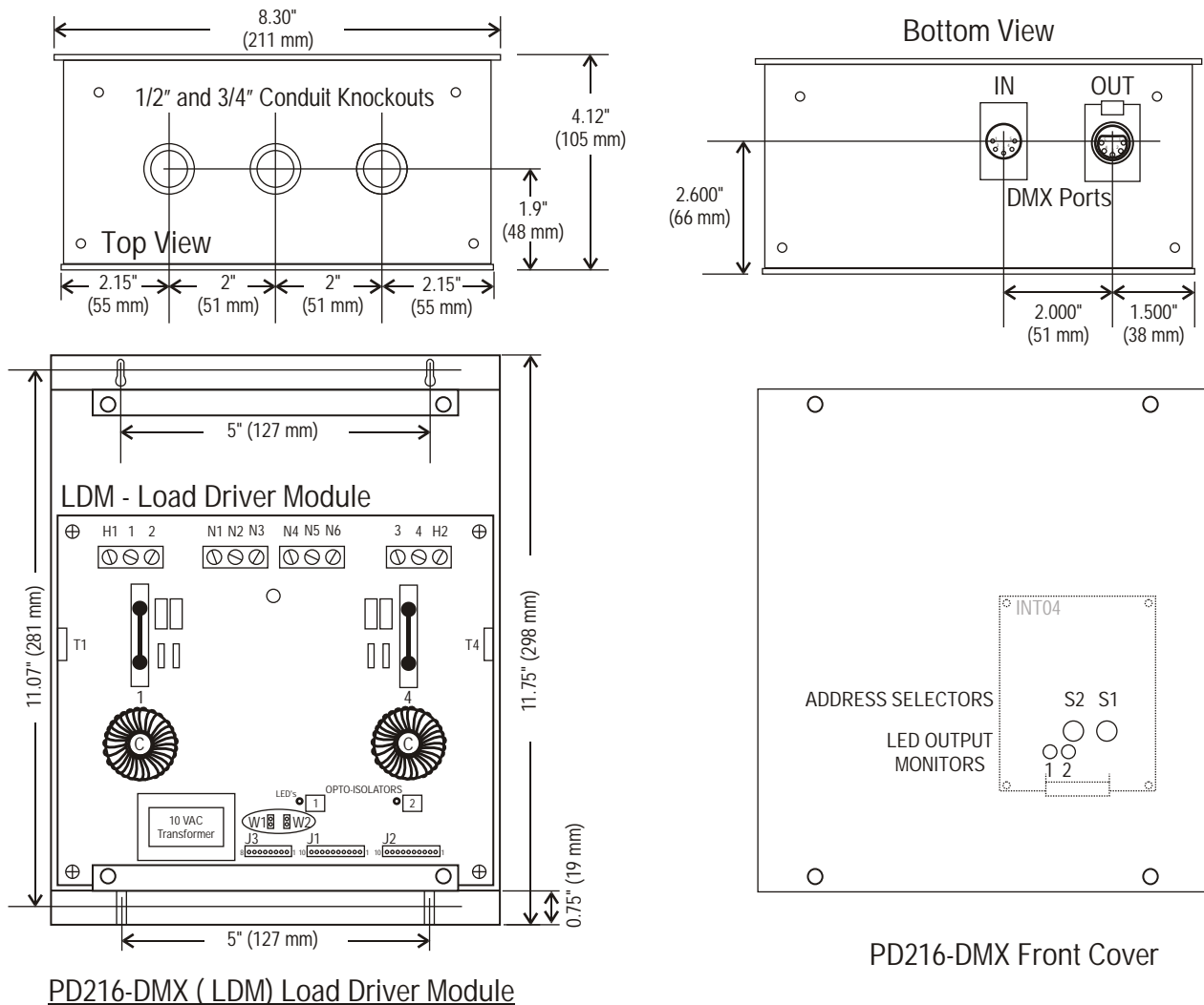
Figure 3 - PD216-DMX Dimensional Diagram
