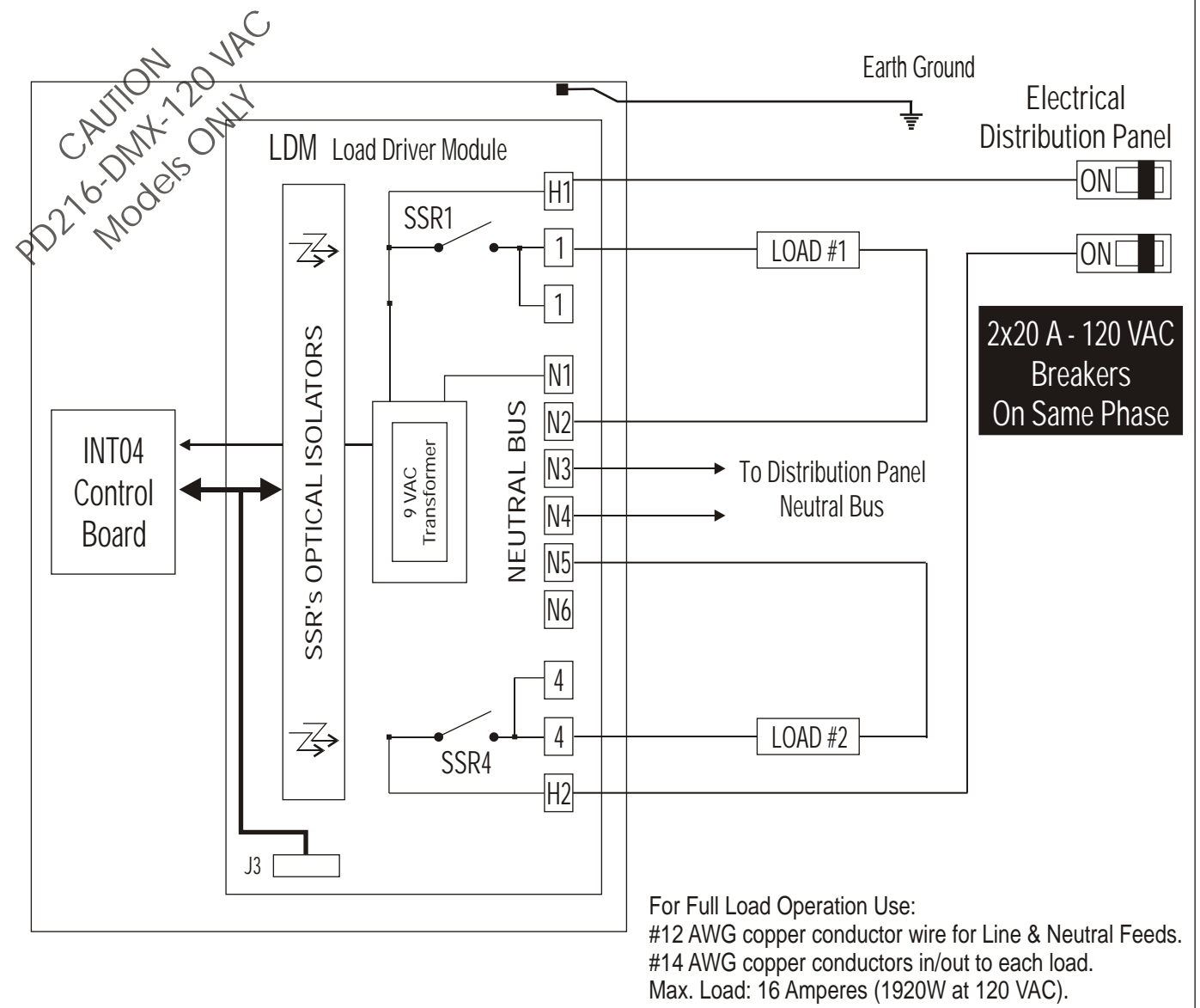
Figure 5 - PD216-DMX Typical 120 VAC Wiring.
